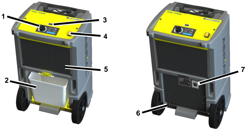
Fig. 2: Back view
